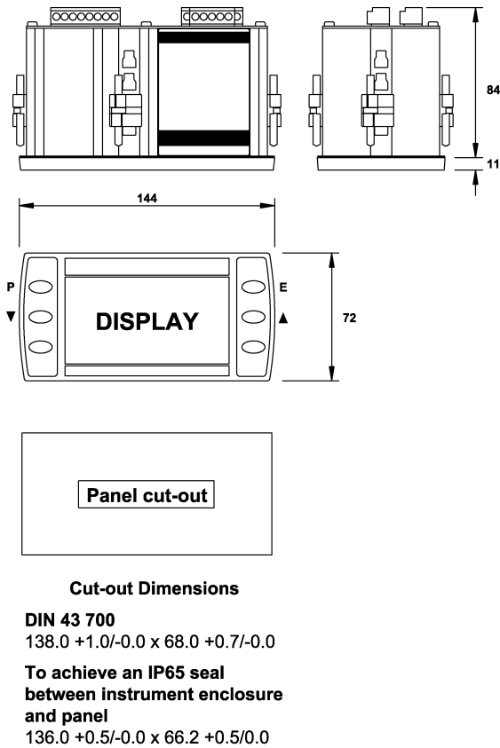
Fig 5 BA488CF-P dimensions
