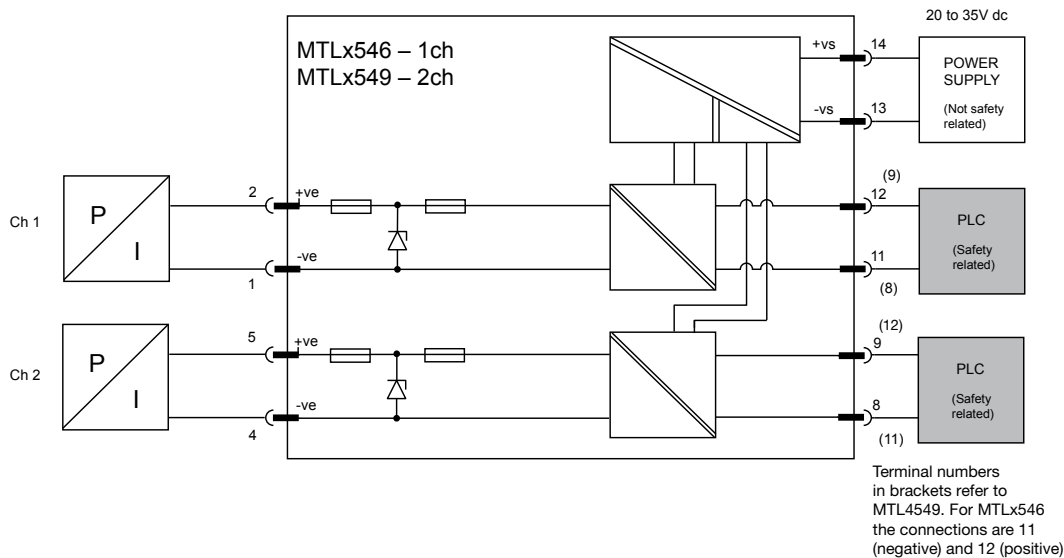
Figure 2.1 – Analogue Output module system configuration – see the ‘Note’ in the text regarding use of dual channel modules
