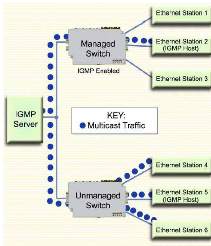
Figure 8-1 IGMP Multicast Filtering Example
