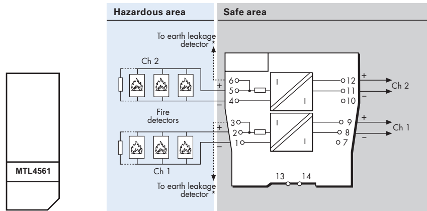
Figure 6.32: Top labels for MTL4561
