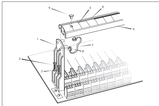
Figure 4.6: Mounting a tagging-strip post
