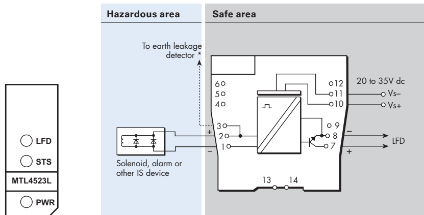
Figure 6.14: Top label for MTL4523L
