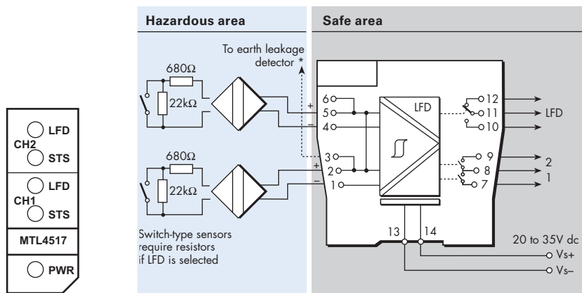
Figure 6.11: Top label for MTL4517
