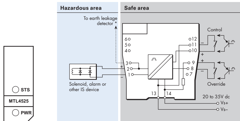
Figure 6.18: Top label for MTL4525
