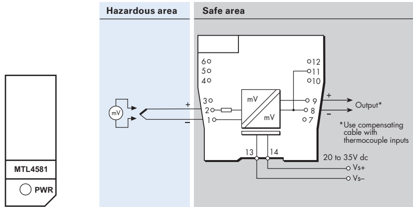
Figure 6.36: Top label for MTL4581
