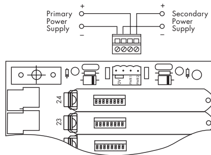
Figure 4.12: PSU connections 24-way
