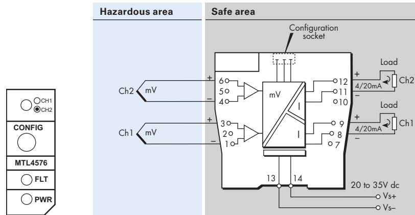
Figure 6.35: Top label for MTL4576
