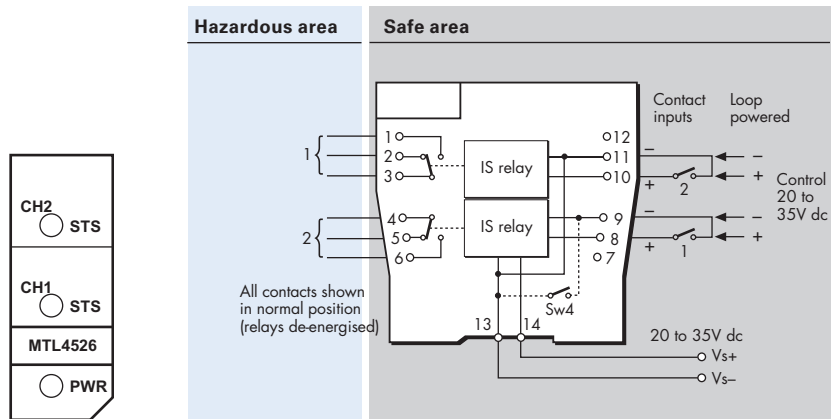
Figure 6.19: Top label for MTL4526
