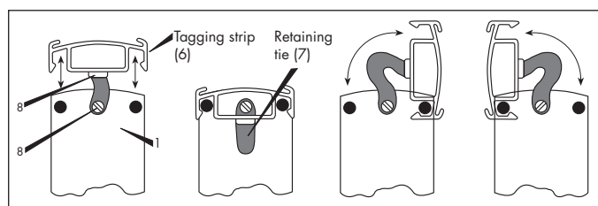
Figure 4.7: Attaching and swivelling a tagging-strip
