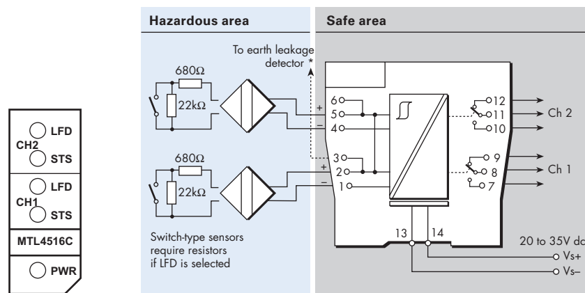
Figure 6.10: Top label for MTL4516C
