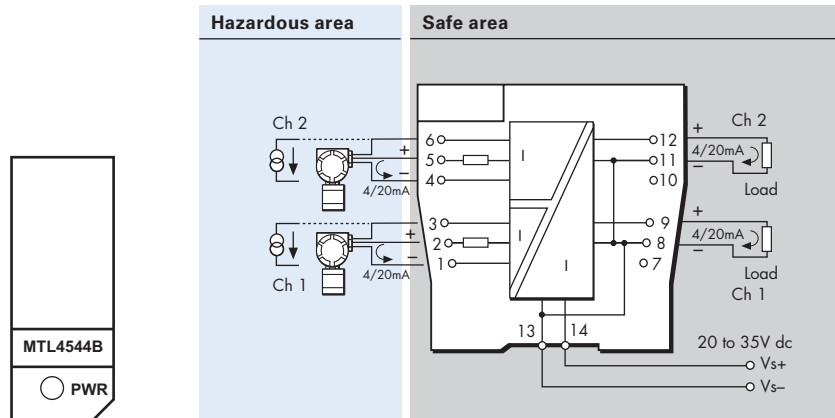
Figure 6.28: Top label for MTL4544B
