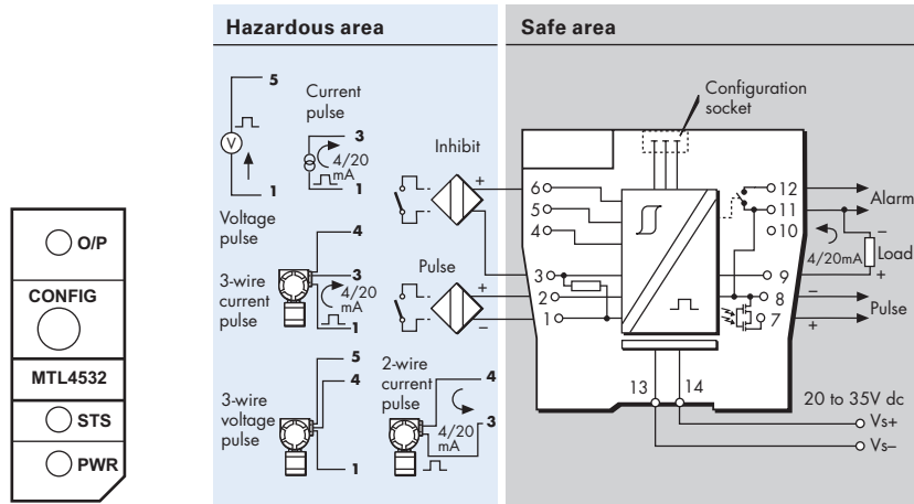
Figure 6.21: Top label for MTL4532
