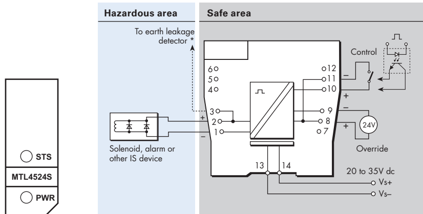
Figure 6.17: Top label for MTL4524S
