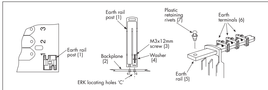
Figure 4.8: Earth rail post kit details
